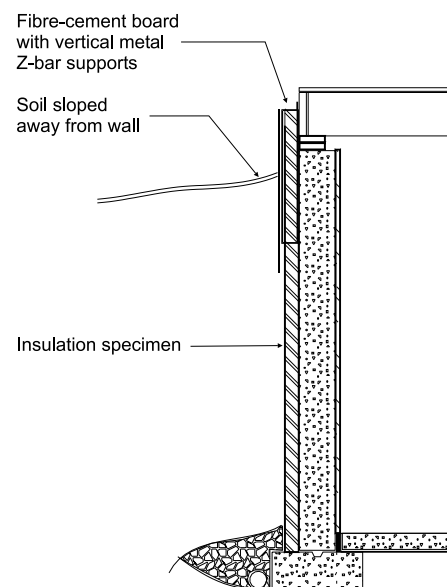
Figure 3. Section of the other experimental basement wall, with vertical metal supports for fibre-cement board and soil sloped away from the wall (good landscaping practice)
