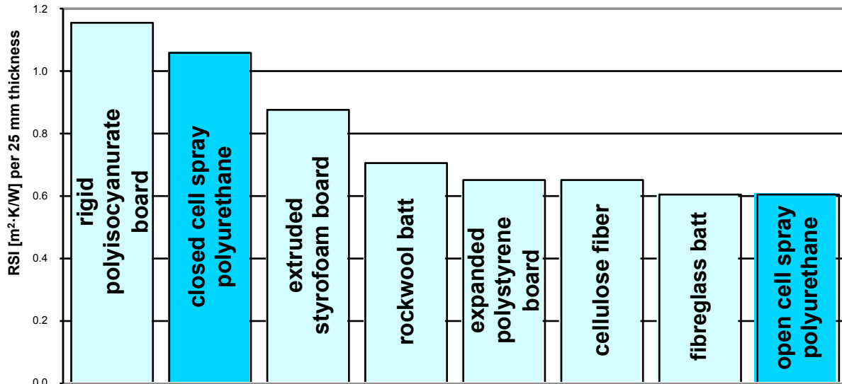
Figure 1.1: Average RSI values of Common Insulation Types (Straube & Burnett 2005)
