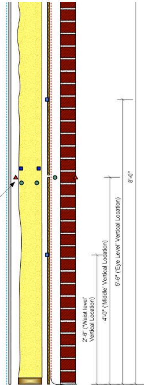
Figure 2.3: Wall Assembly 6 (1/2 pcf open cell SPF)
